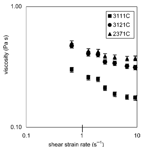
Figure 1. Viscosity curves on log–log axes for zein samples in DMF at 25% protein and 25 °C at various shear rates.
