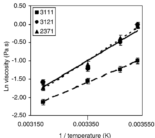
Figure 3. Viscosity vs temperature for 25% zein DMF solutions after 15 min at specific temperatures at 2.64 s -1 . Equations for fitted lines are as follows: lot 3121 (solid line) is y = 4575 (1/K) - 16.3 and R^2 = 0.94 ; lot 2371 (dotted line) is y = 5010 (1/K) - 17.8 and R^2 = 0.99 ; and lot 3111 (dashed line) is y = 3240 (1/K) - 12.5 and R^2 = 0.99 .
