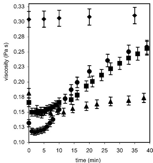
Figure 4. Viscosity of 25% lot 3121 zein in DMF solutions at 2.64 s -1 measured at various times at different temperatures: ◆, 25 °C; ▲, 40 °C; ■, 48 °C; and ●, 55 °C.
