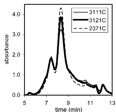
Figure 6. SEC analysis of zein lots. Traces were normalized so that the areas under the curves are the same. Lot 3121 was the only material that had material eluting from the column in less than 6 min.
