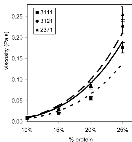
Figure 2. Viscosity vs % protein for zeins at 25 °C in DMF at 13.2 s^{-1} . Equations for fitted lines are as follows: lot 3111 (dotted line) is y = 13.40 (% protein 3.29 ) and R^2 = 0.97 ; lot 3121 (solid line) is y = 18.62 (% protein 3.30 ) and R^2 = 0.98 ; and lot 2371 (dashed line) is y = 20.98 (% protein 3.31 ) and R^2 = 0.97 .
