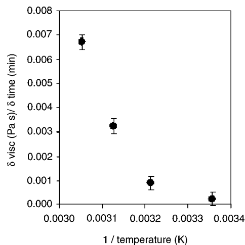
Figure 5. Plot of rate of viscosity increase for 25% lot 3121 zein in DMF solutions vs reciprocal temperature (K).
